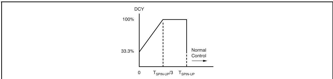
Figure 24. Spin-Up Process
