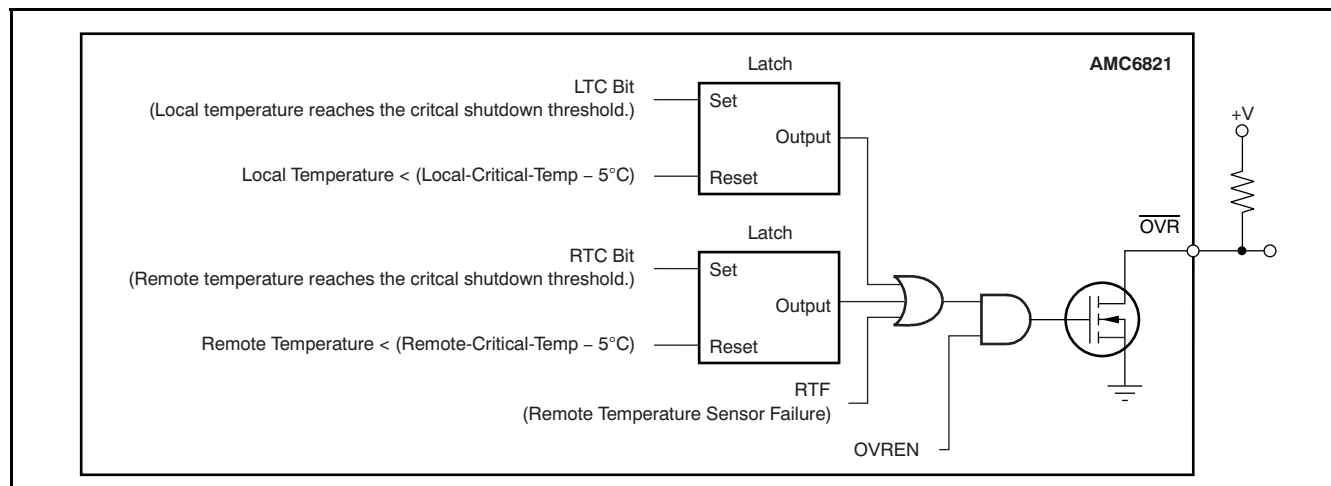
Figure 30. \overline{\text{OVR}} Pin
