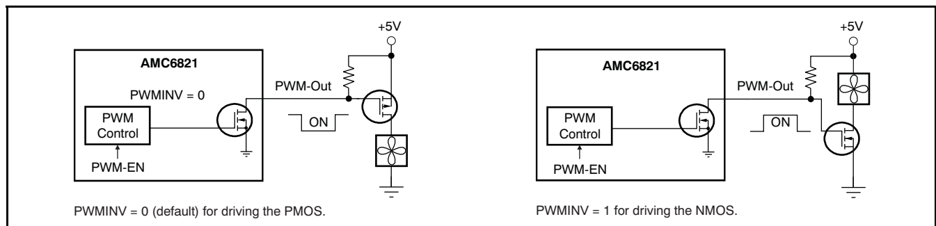
Figure 15. PWM Output
