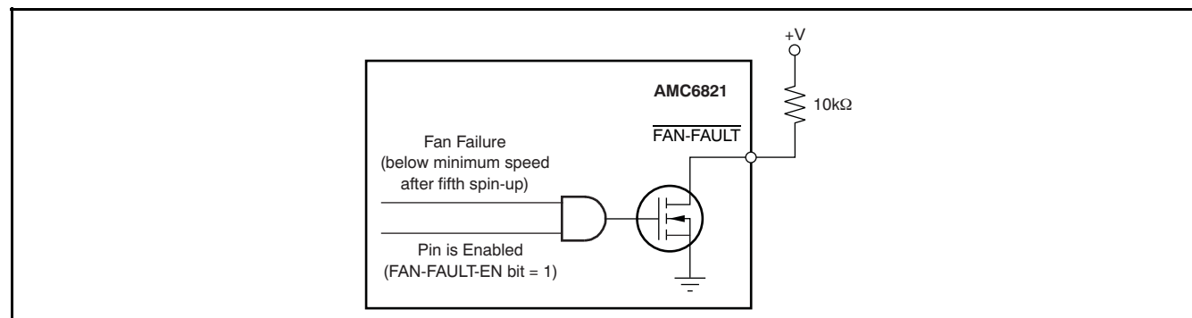
Figure 21. \overline{\text{FAN-FAULT}} Pin
