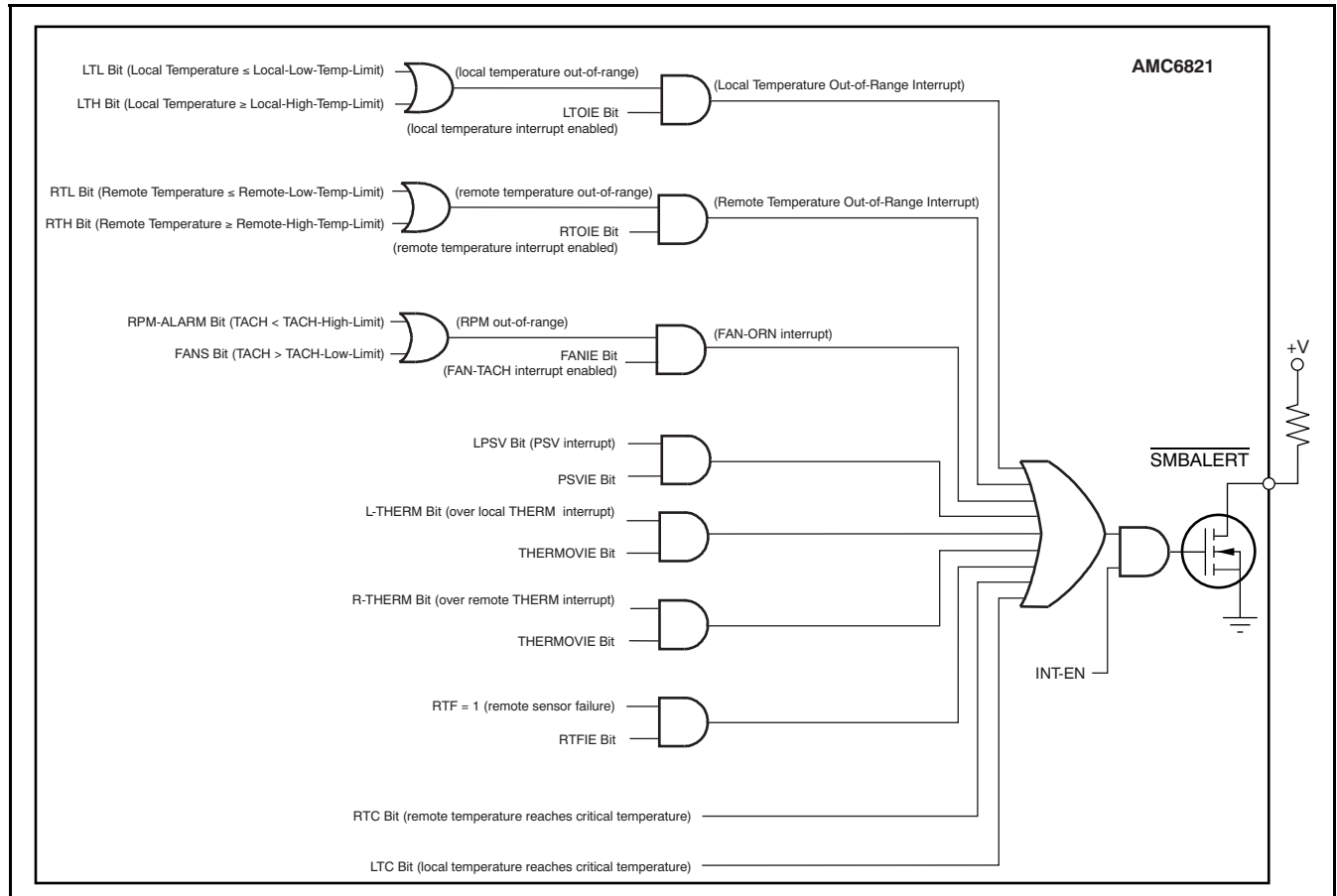
Figure 33. SMBALERT
